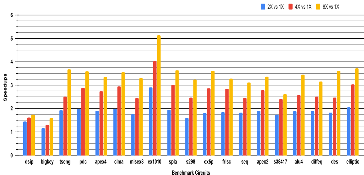
FIGURE 5: Speedups of each benchmark using ParaLaR when running it with 2, 4 and 8 threads.
